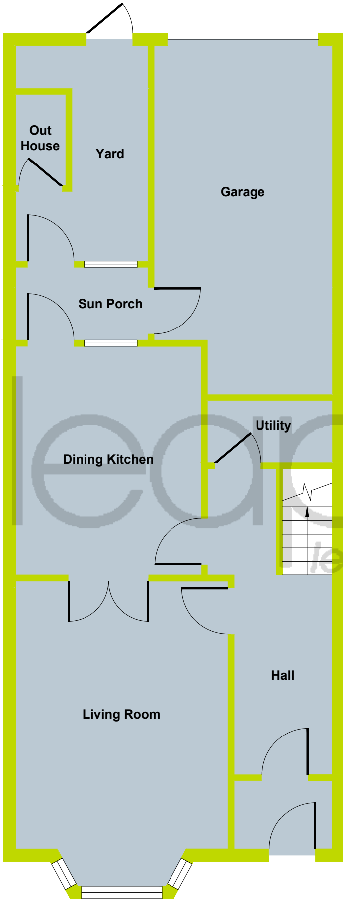
Ground Floor
