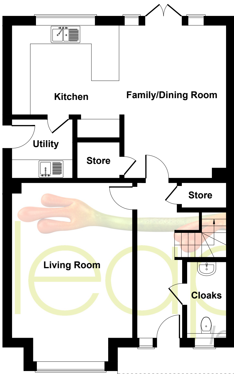
GROUND FLOOR
