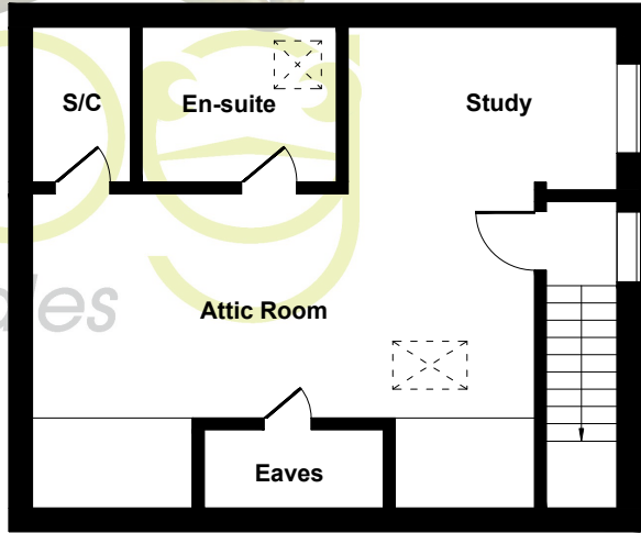
ATTIC FLOOR
